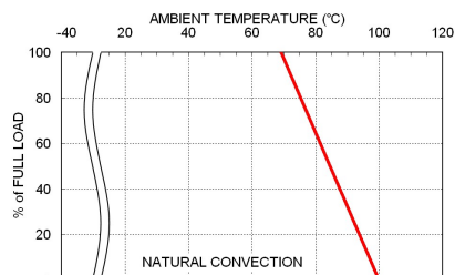
FKC08-48S05 Derating Curve
