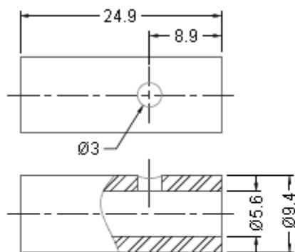
HANDLE
